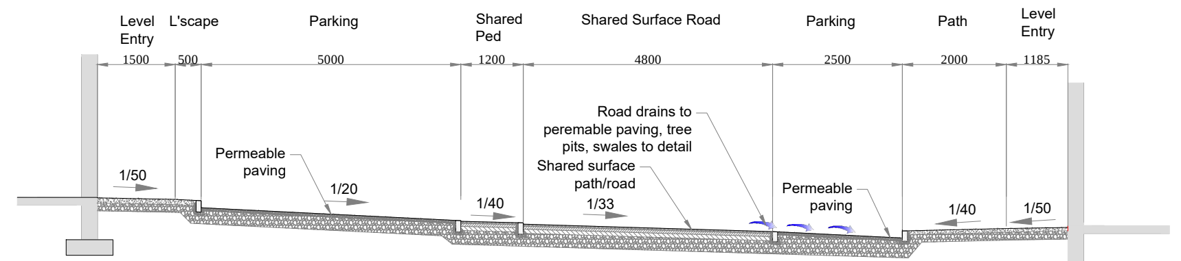
TYPICAL STREET SECTION Scale 1:100
